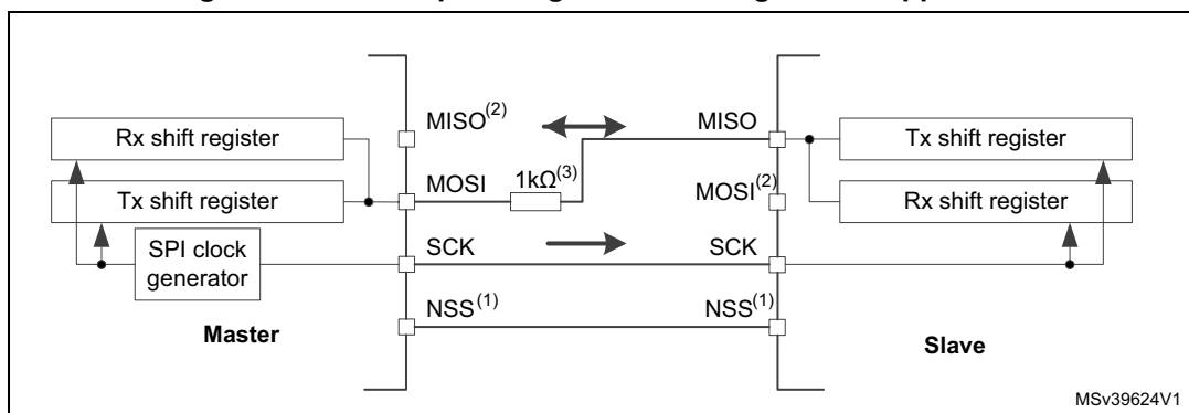
Figure 275. Half-duplex single master/ single slave application
