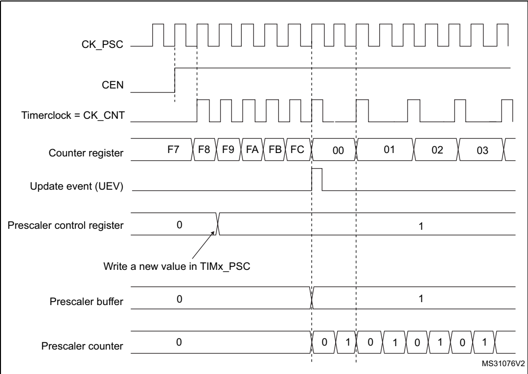
Figure 202. Counter timing diagram with prescaler division change from 1 to 2
