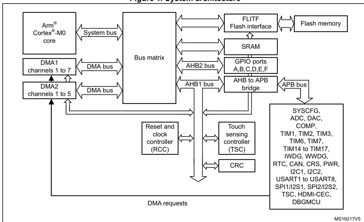
Figure 1. System architecture
