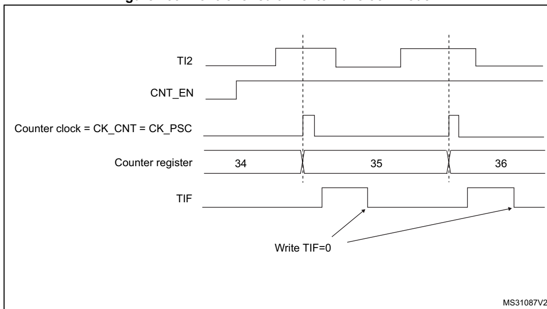
Figure 133. Control circuit in external clock mode 1
