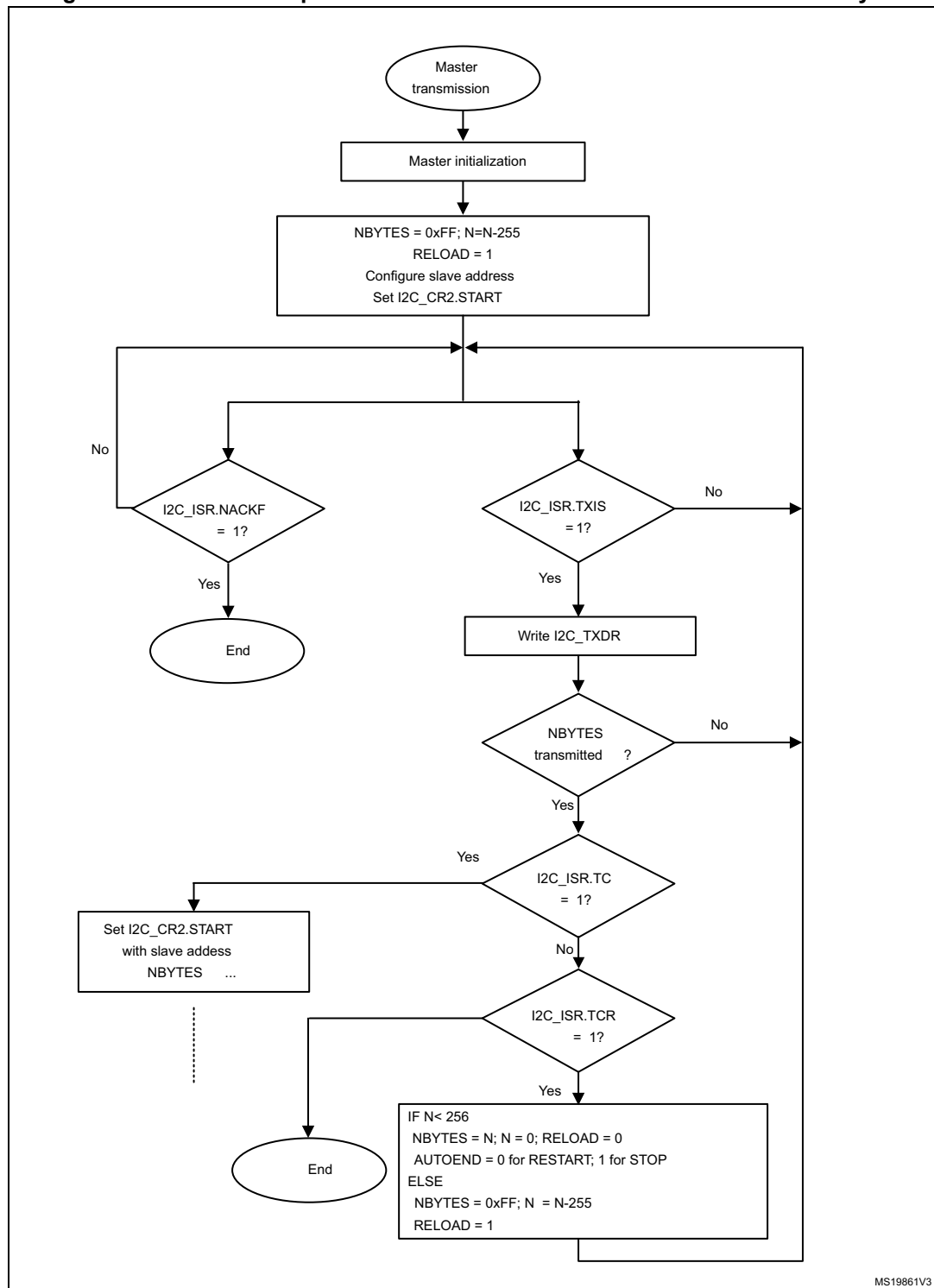
Figure 236. Transfer sequence flow for I2C master transmitter for N &gt; 255 bytes
