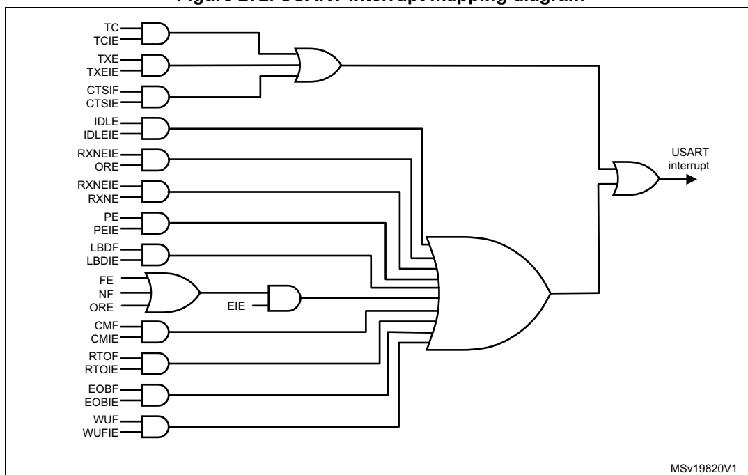
Figure 272. USART interrupt mapping diagram
