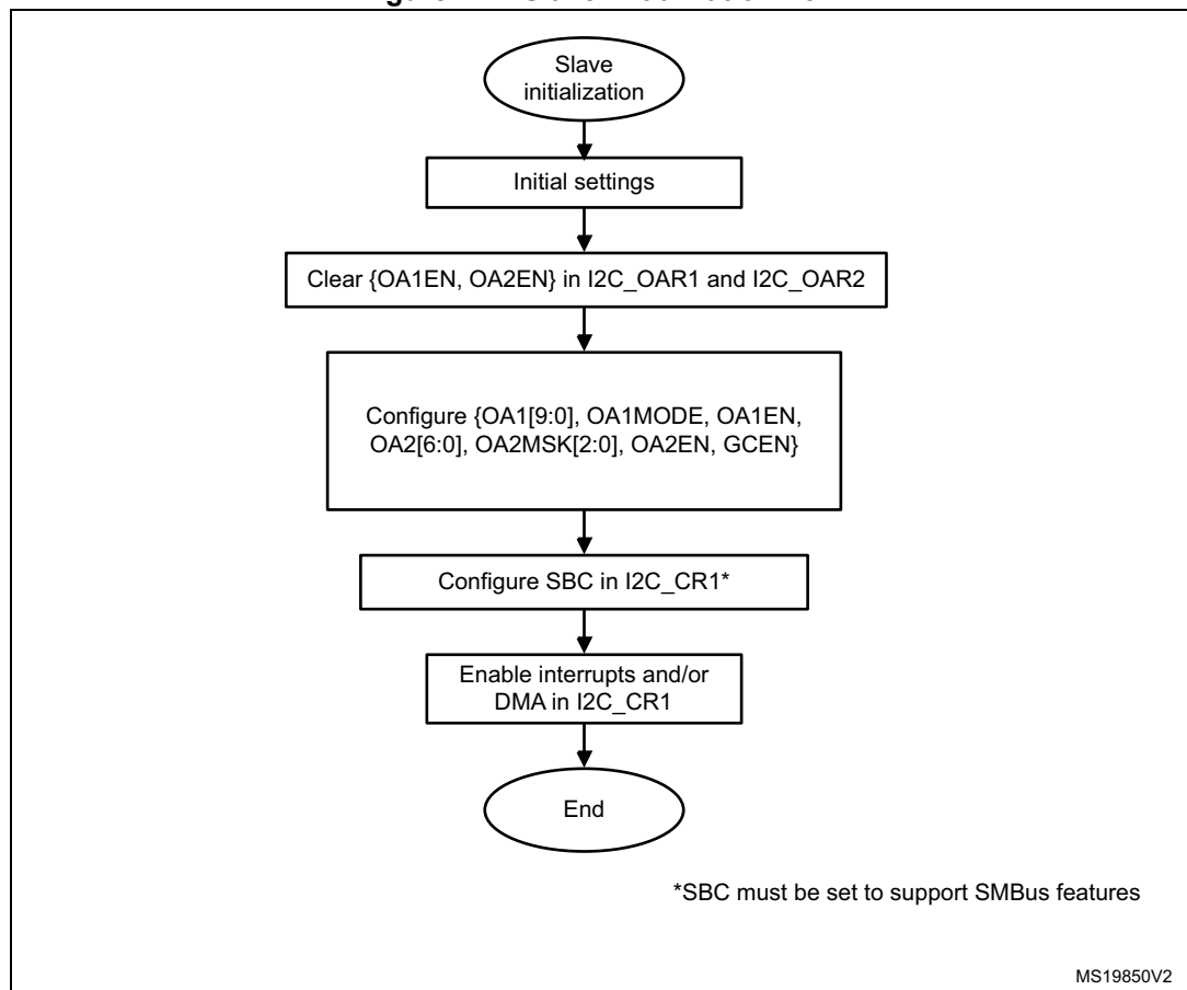
Figure 224. Slave initialization flow
