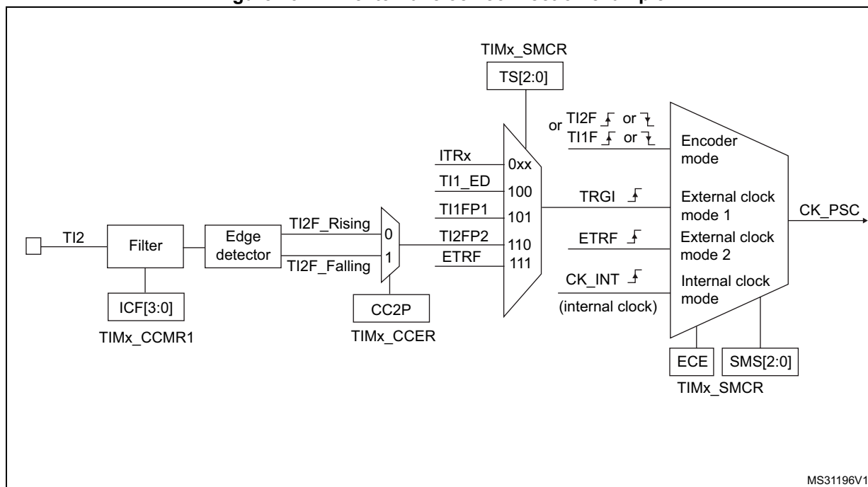
Figure 132. TI2 external clock connection example
