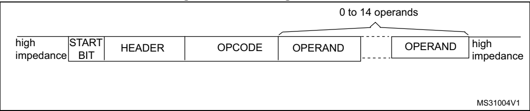
Figure 330. Message structure
