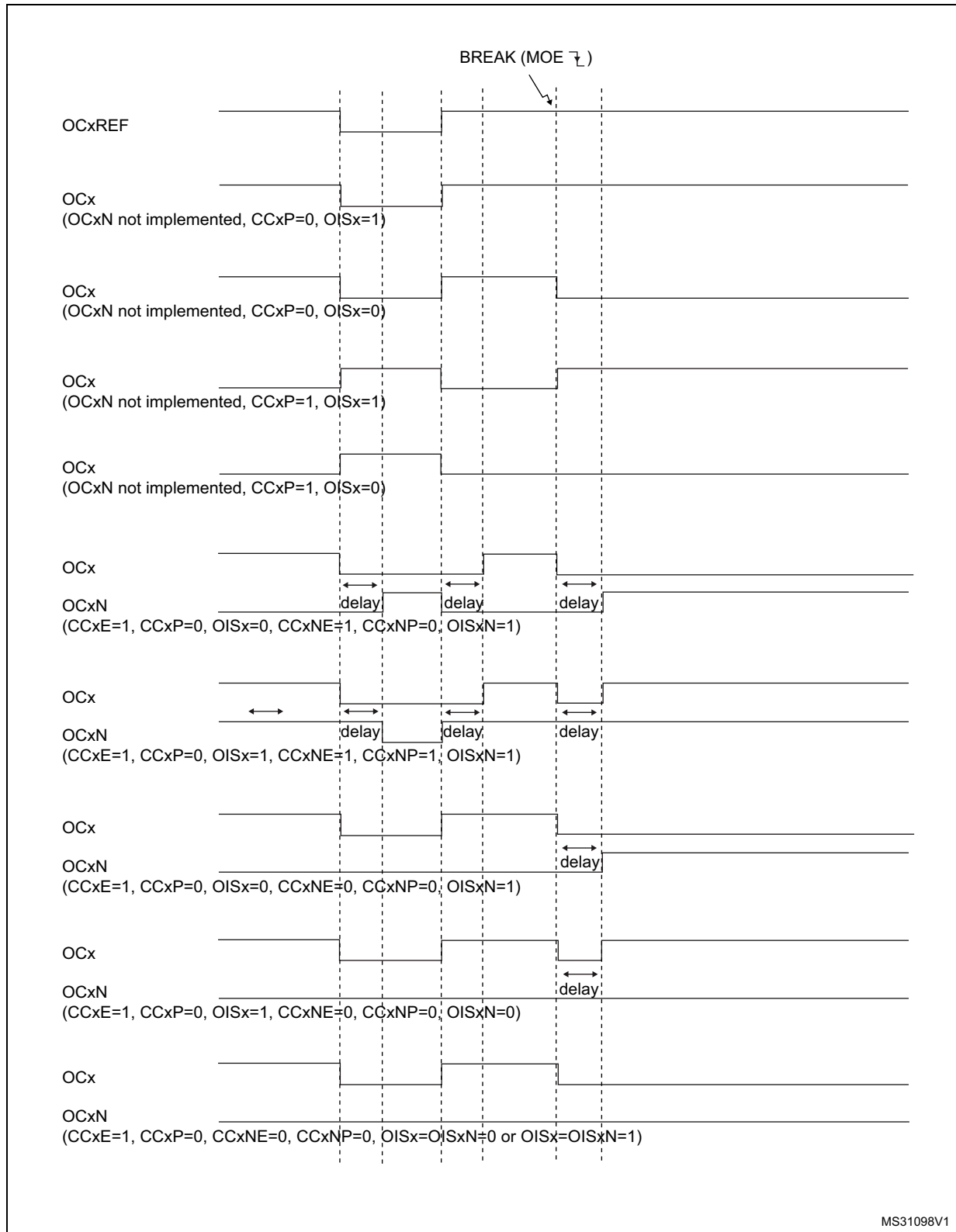
Figure 196. Output behavior in response to a break
