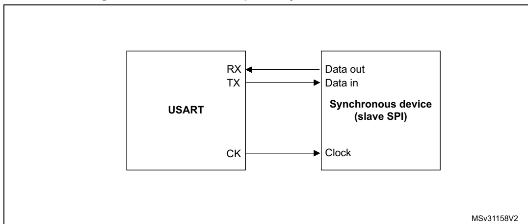
Figure 259. USART example of synchronous transmission
