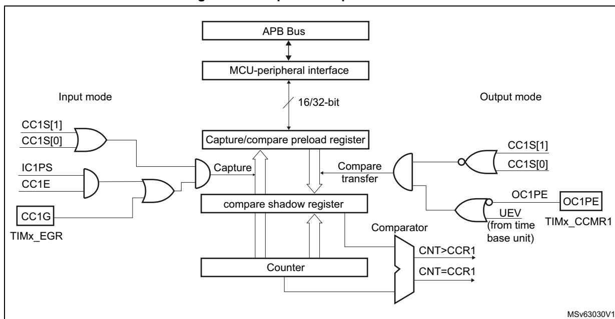
Figure 168. Capture/compare channel 1 main circuit
