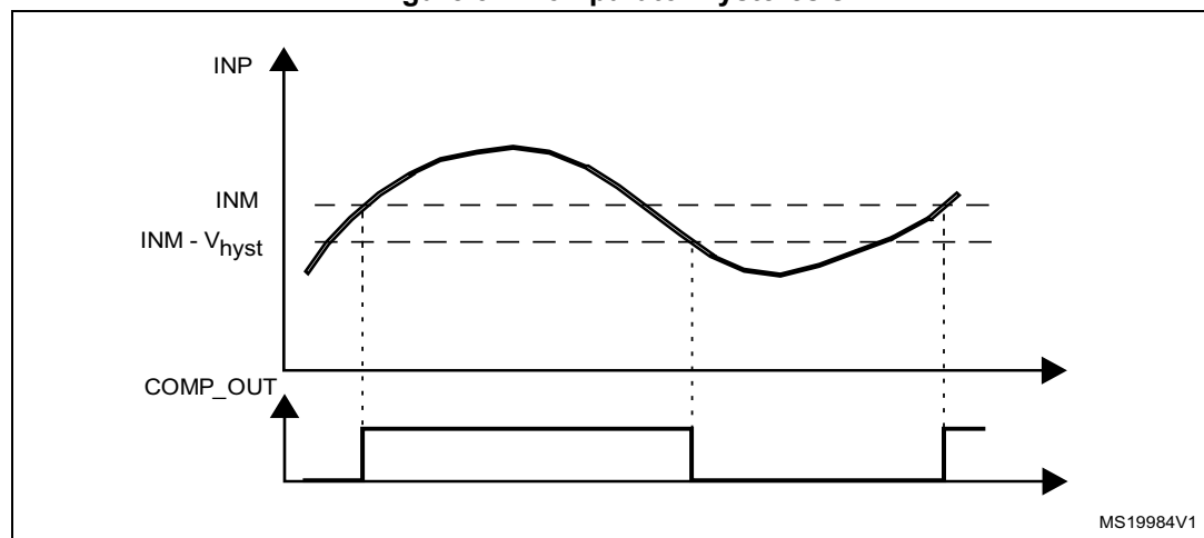
Figure 57. Comparator hysteresis
